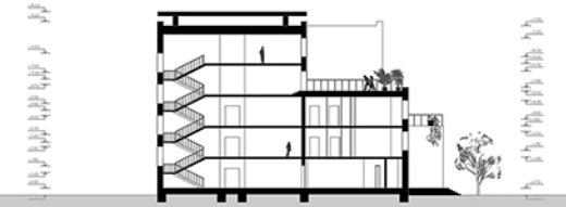
SECTION 2-2
