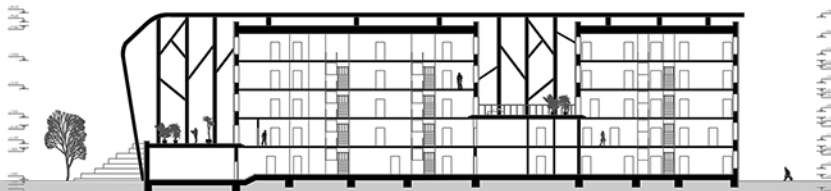
SECTION 1-1
